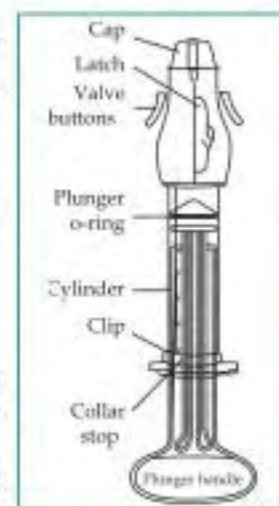
Figure 4: MVA Plus Aspirator
